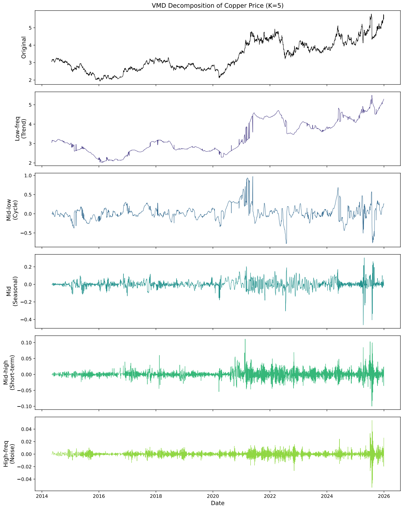
Fig. 8: Variational Mode Decomposition of the copper price series into K = 5 frequency-band modes.
