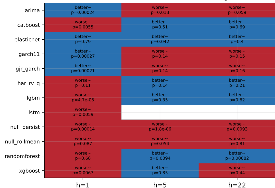
T1 DM test vs har_rv
