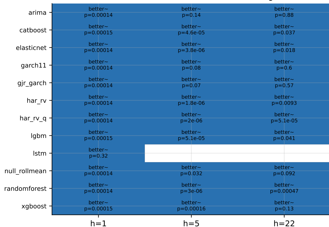
T1 DM test vs null_persist
