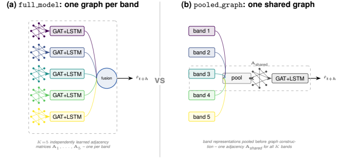
Fig. 3: The RQ1 comparison made visible: (a) full_model builds a separate learned graph per frequency band; (b) pooled_graph pools band representations before constructing a single shared graph. Section V-E1 shows that in the trained model, (a)’s five graphs collapse to a near-uniform adjacency indistinguishable from one another, which is why the ablation in Table VIII does not show a clean advantage for (a) over (b).
