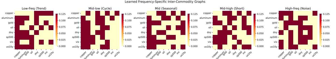
Fig. 6: Learned adjacency matrices for each of the five VMD frequency bands.
