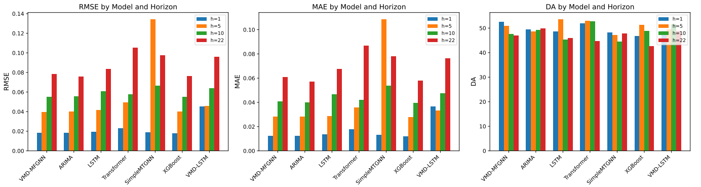
Fig. 1: RMSE, MAE, and Directional Accuracy by model and horizon, for VMD-MFGNN and the six baselines.
