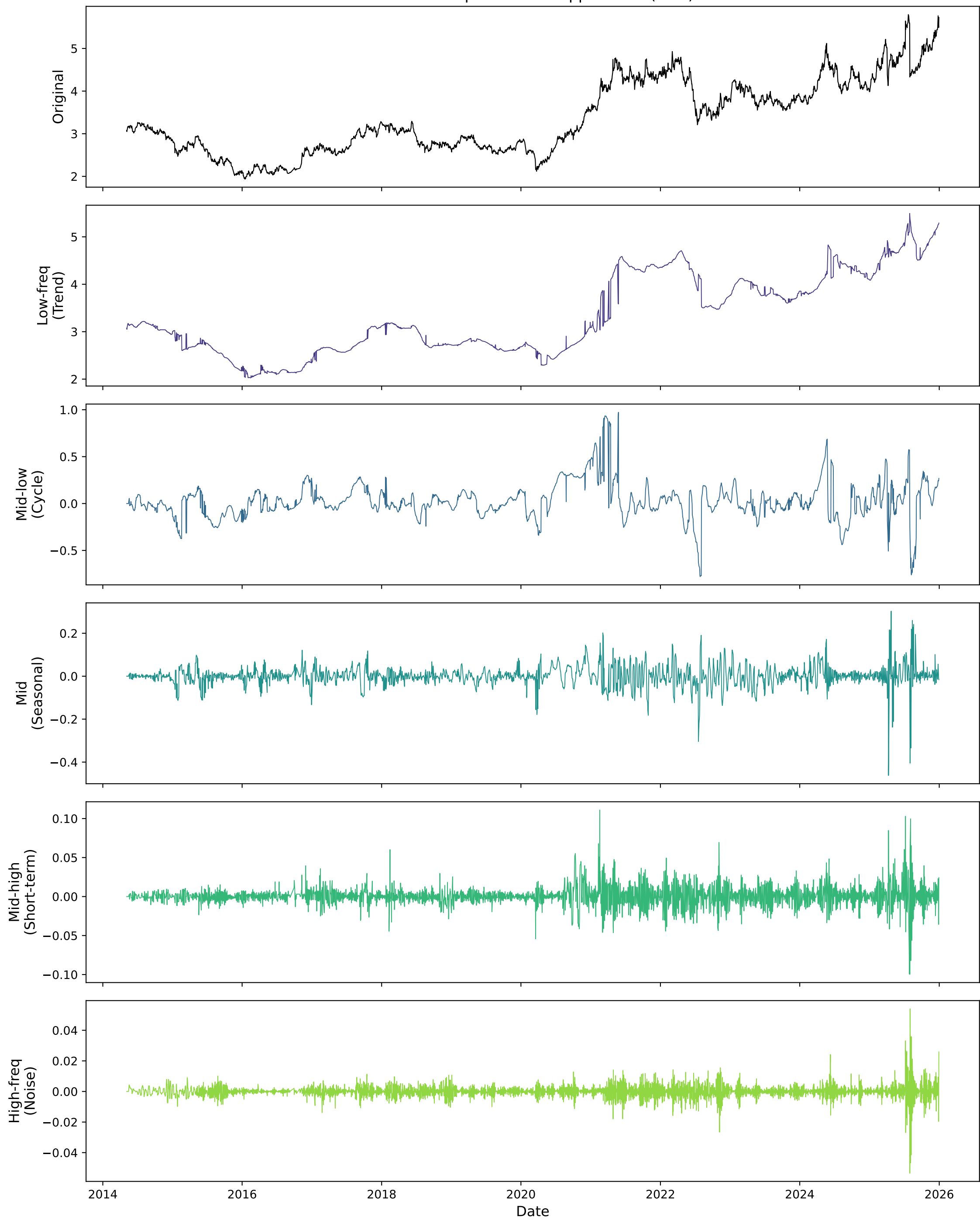
VMD Decomposition of Copper Price (K=5)
