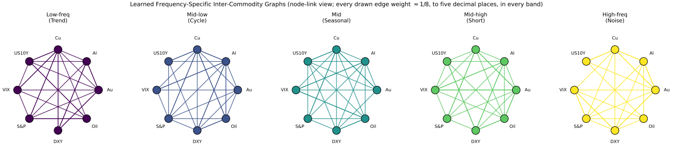
Fig. 6: Node-link rendering of the same five learned adjacency matrices shown in Figure 5, from the identical saved learned_graphs.pt data. Node layout is a fixed circle, identical across bands, so only edge presence and opacity vary; the visual near-identity of all five panels is the collapse finding made directly legible.
