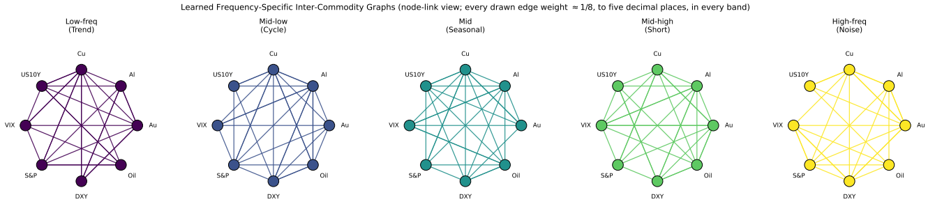
Fig. 7: Node-link rendering of the same five learned adjacency matrices shown in Figure 6, from the identical saved learned_graphs.pt data. Node layout is a fixed circle, identical across bands, so only edge presence and opacity vary; the visual near-identity of all five panels is the collapse finding made directly legible.
