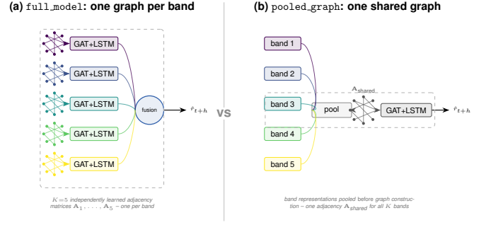
Fig. 3: The RQ1 comparison made visible: (a) full_model builds a separate learned graph per frequency band; (b) pooled_graph pools band representations before constructing a single shared graph. Section V-E1 shows that in the trained model, (a)’s five graphs collapse to a near-uniform adjacency indistinguishable from one another, which is why the ablation in Table VIII does not show a clean advantage for (a) over (b).
