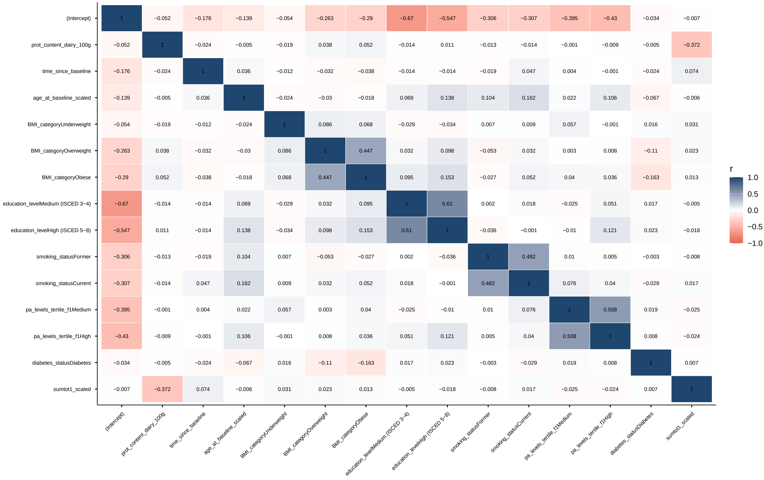
Fixed-Effect Correlations – HGS_MAX ~ prot_content_dairy_100g (linear) | main
