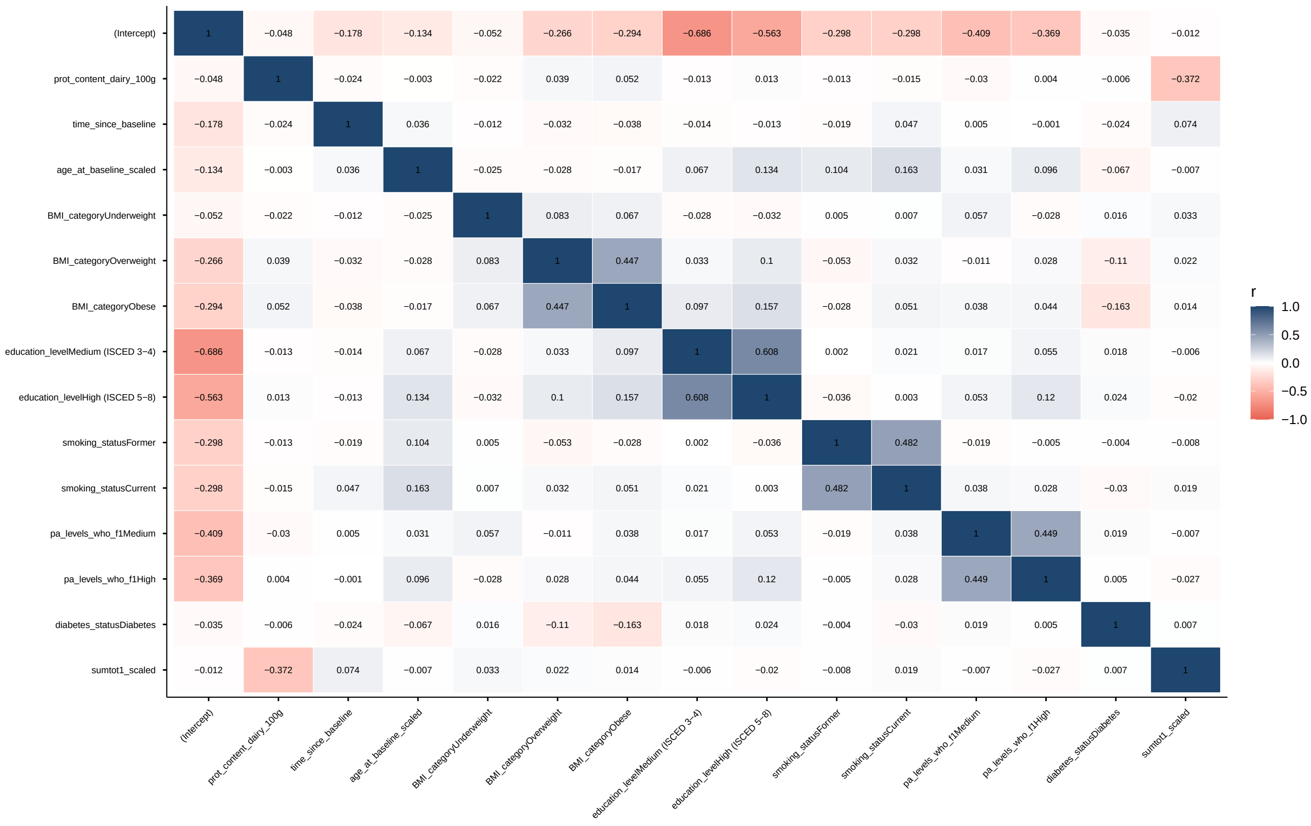
Fixed-Effect Correlations – HGS_MAX ~ prot_content_dairy_100g (linear) | other_PA
