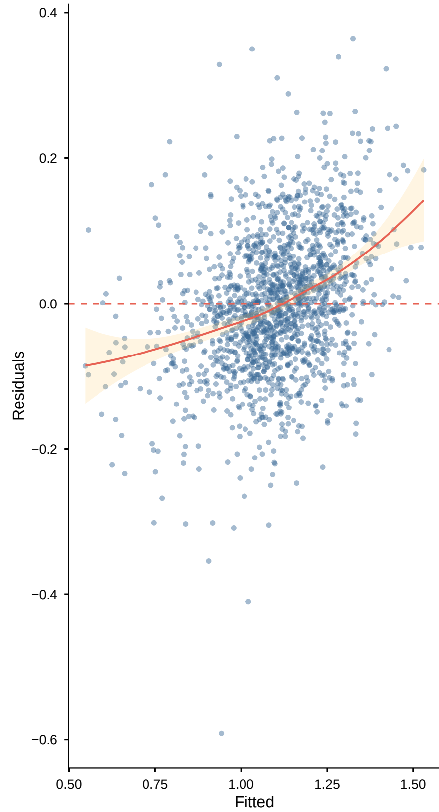
A Residuals vs Fitted M10 Poly 2 age
