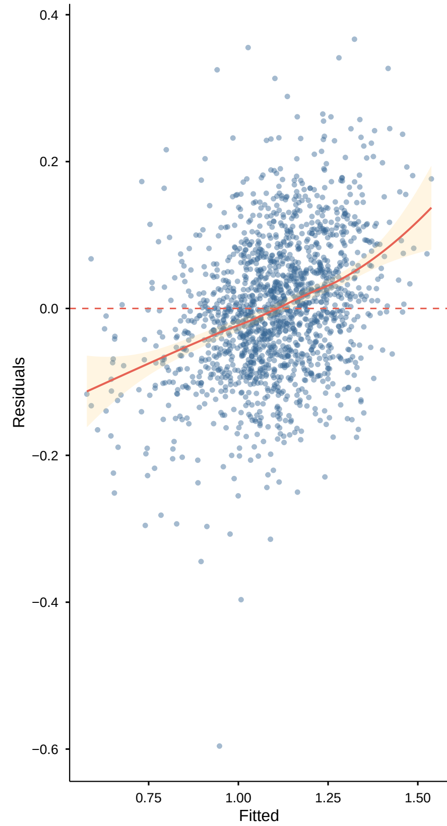
A Residuals vs Fitted M4 Dairy × time
