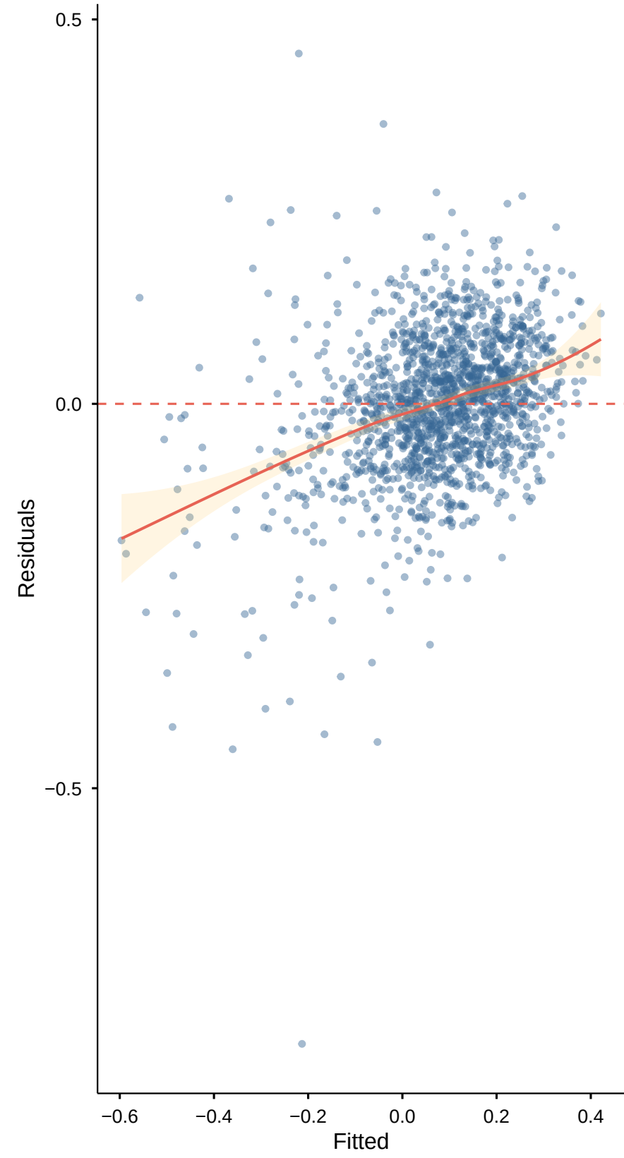
A Residuals vs Fitted M3a Log outcome
