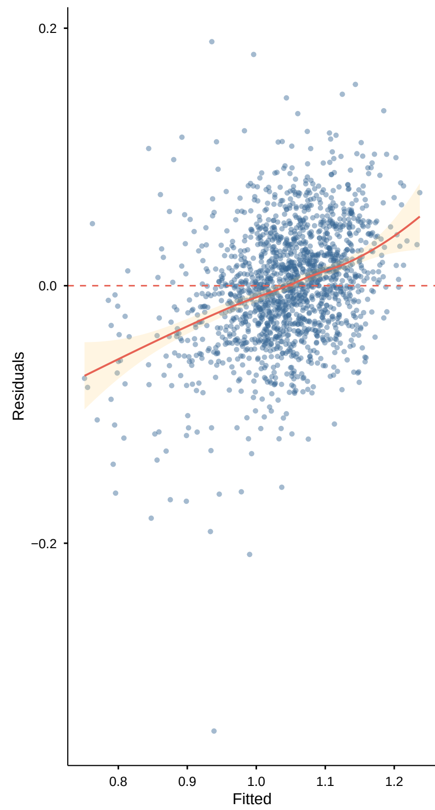
A Residuals vs Fitted M3b Sqrt outcome
