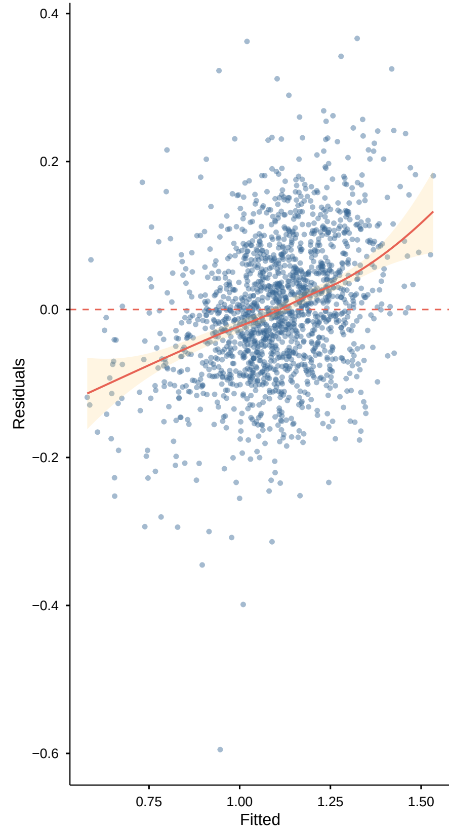
A Residuals vs Fitted M2 Poly 2 dairy
