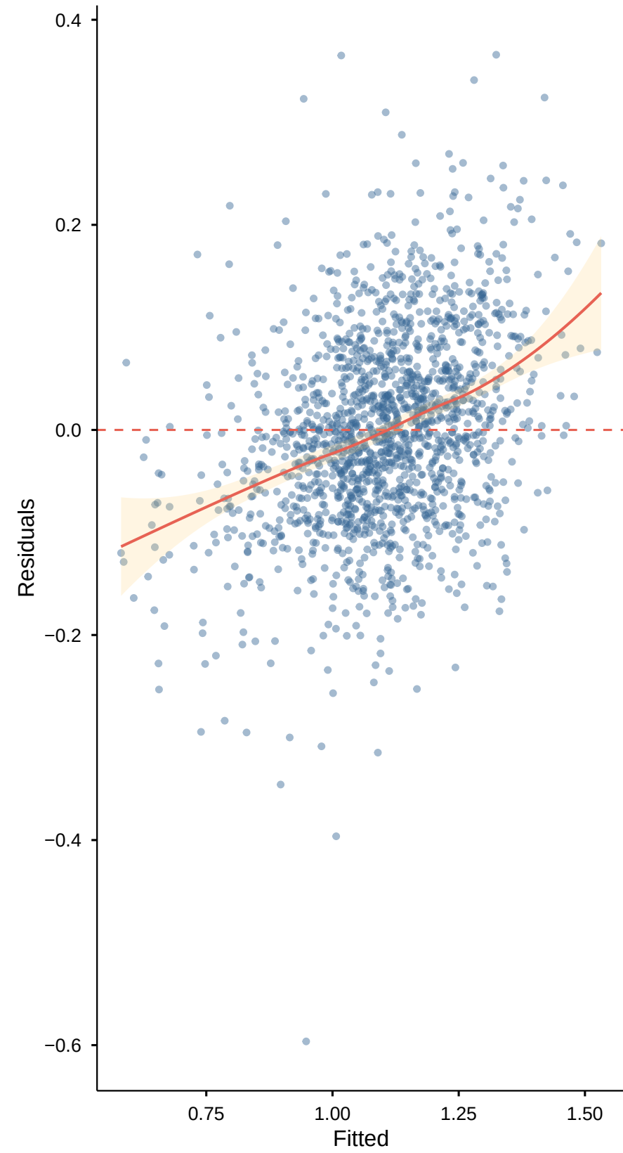
A Residuals vs Fitted M1 NS spline dairy
