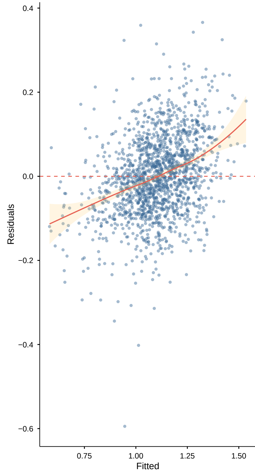
A Residuals vs Fitted M6 Within-/between dairy
