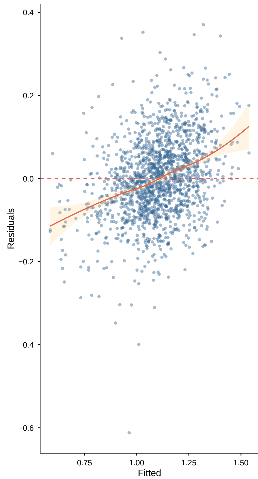
A Residuals vs Fitted M5 Height + Weight
