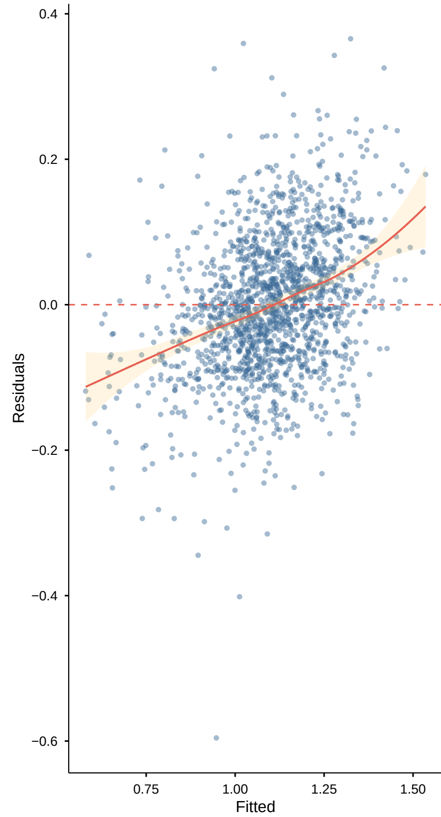
A Residuals vs Fitted M0 Reference
