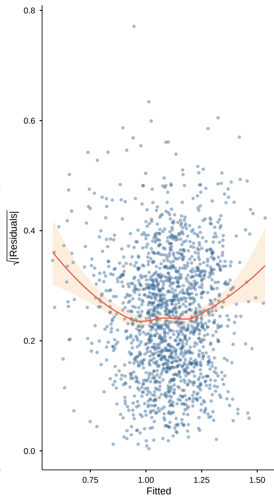
B Scale-Location
