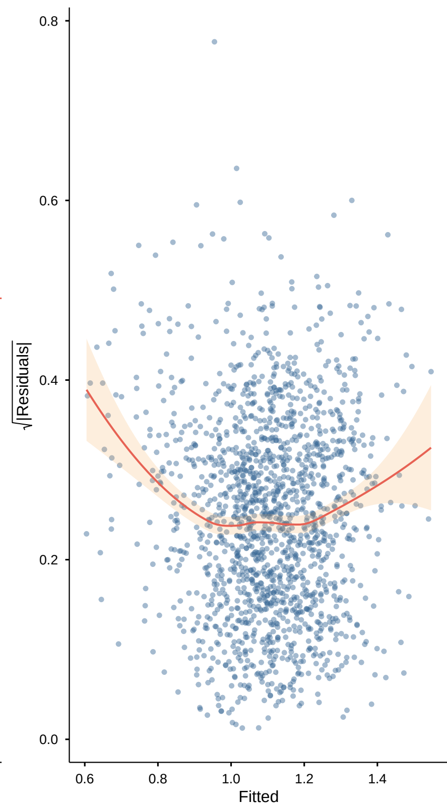
B Scale-Location
