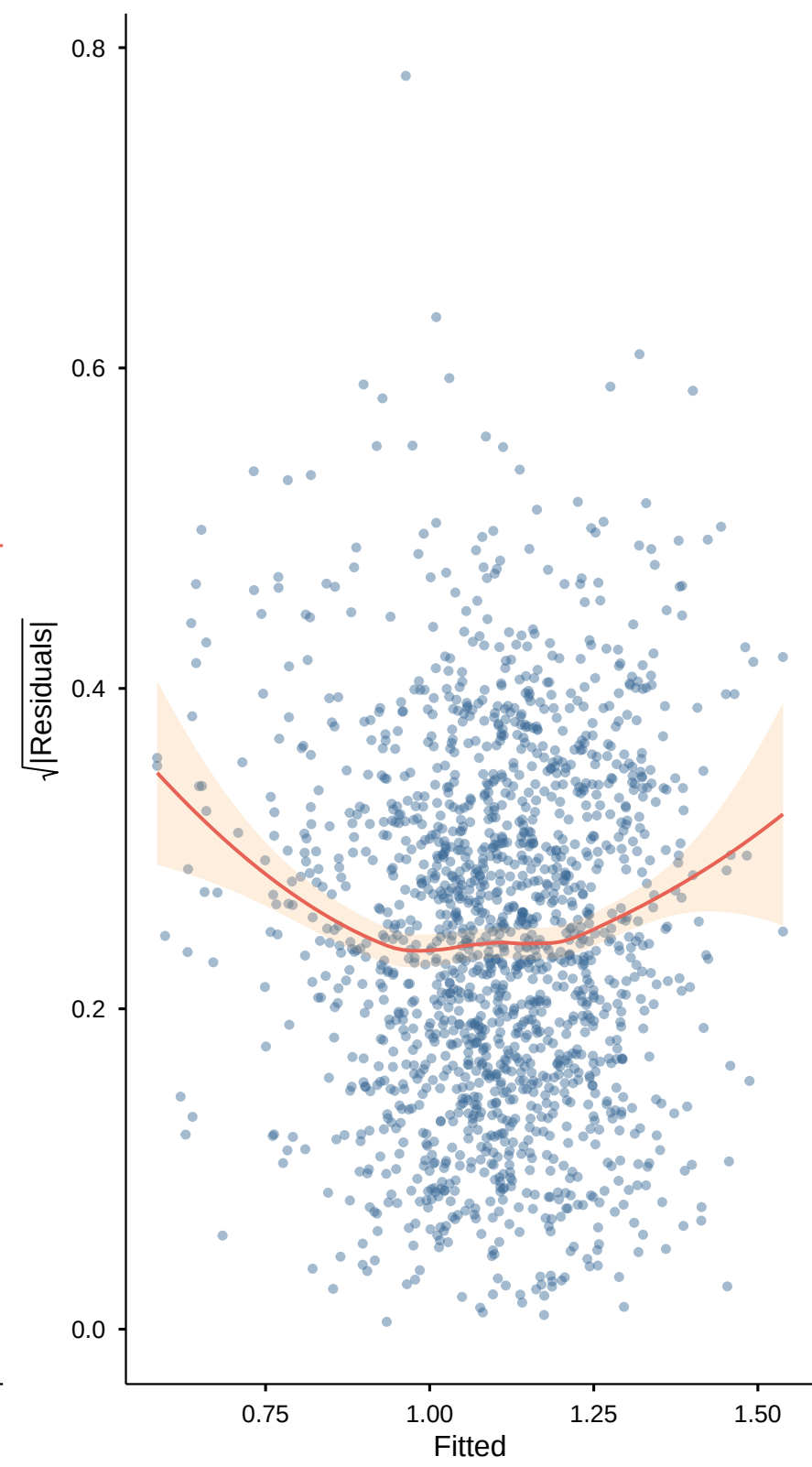
B Scale-Location
