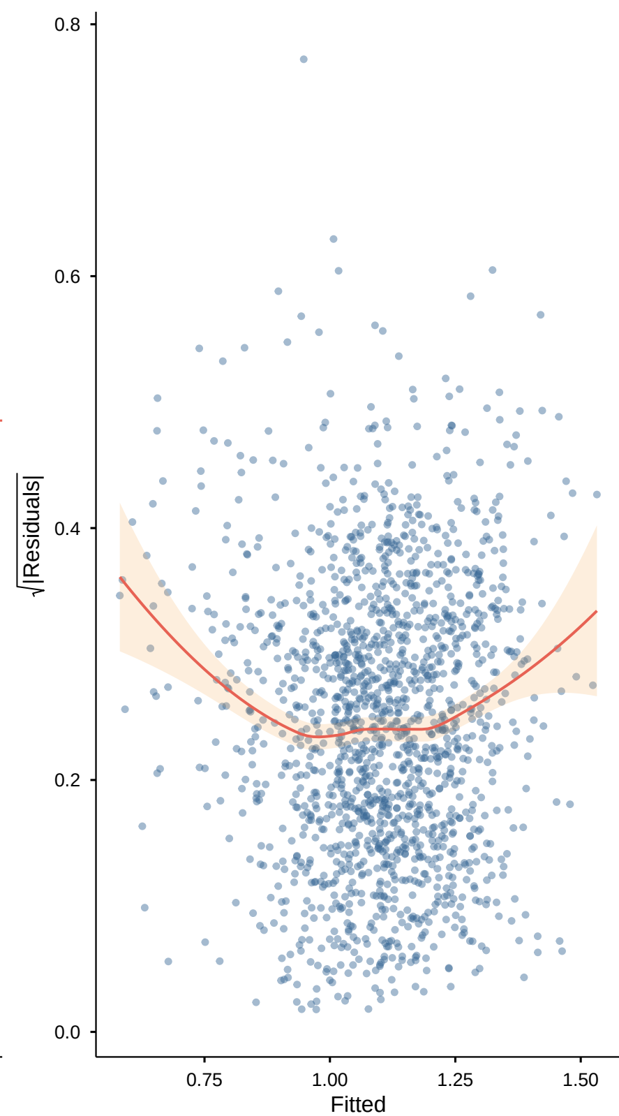
B Scale-Location
