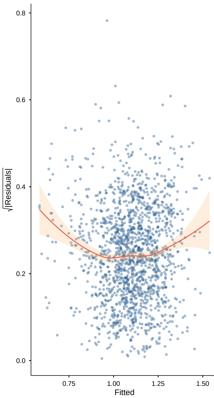
B Scale-Location
