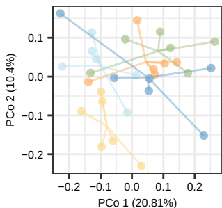
Rhizosphere – NPK soil
