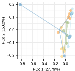
Root – PK soil
