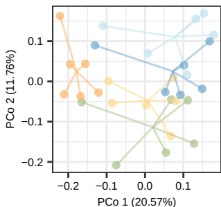
Rhizosphere – PK soil
