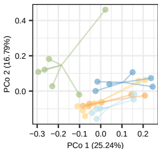
Root – NPK soil
