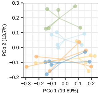
Root – UF soil
