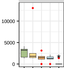
Formononetin (F903)
