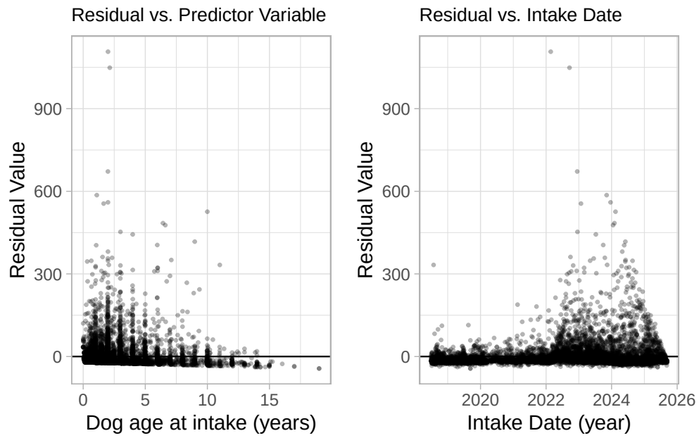
Figure 2: Residual diagnostic plots for linear regression model predicting a dog's length of stay based on their age at intake. Unequal variances are observed in the left-hand plot and a clear non-linear shape is seen in the right-hand plot.
