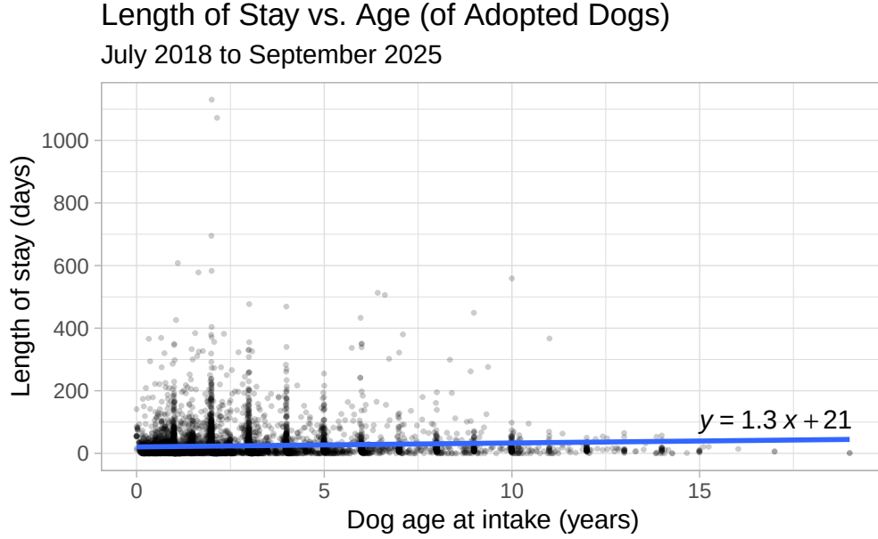
Figure 1: Scatterplot of dog age at intake versus their length of stay for adopted dogs. The fitted linear model, y = 1.3x + 21 ) indicates a slight positive association.
