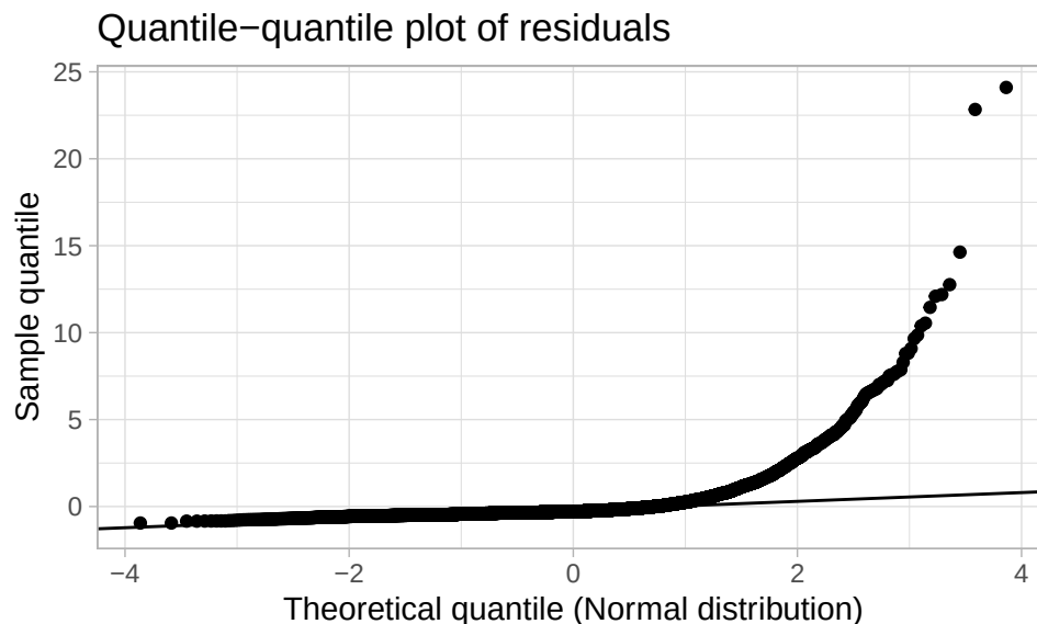
Figure 3: Diagnostic Q-Q plot indicates non-normality of residuals as seen by the right-end points curving upward away from the reference line.
