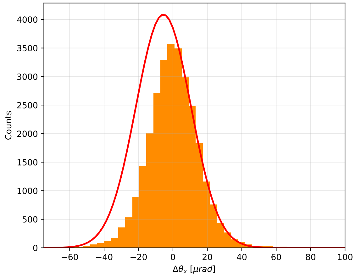
\Delta\theta_x distribution - ( \theta_b = 50 \mu\text{rad} )
