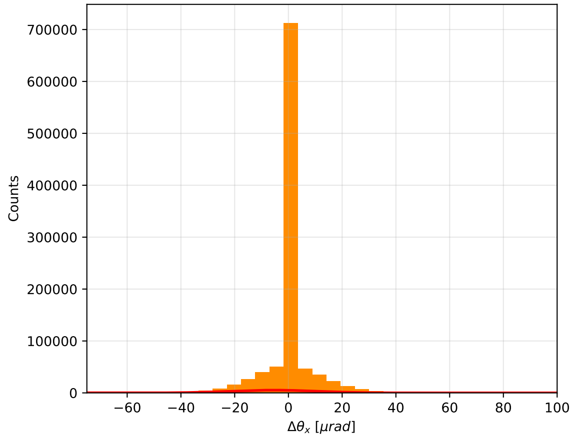
\Delta\theta_x distribution - (survived particles)
