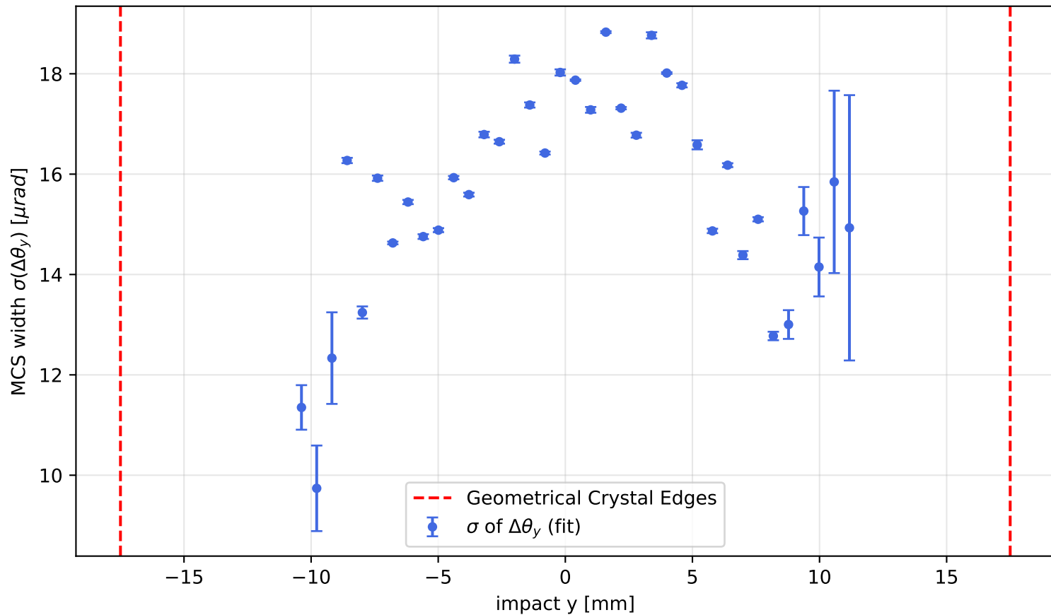
Material Edge Transition - y plane
