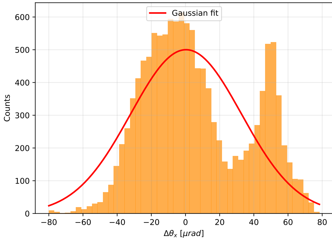
Inside crystal — pos = -0.02 mm, n = 12728
