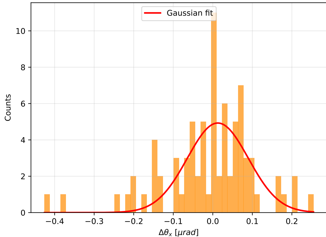
Outside crystal — pos = -2.09 mm, n = 79
