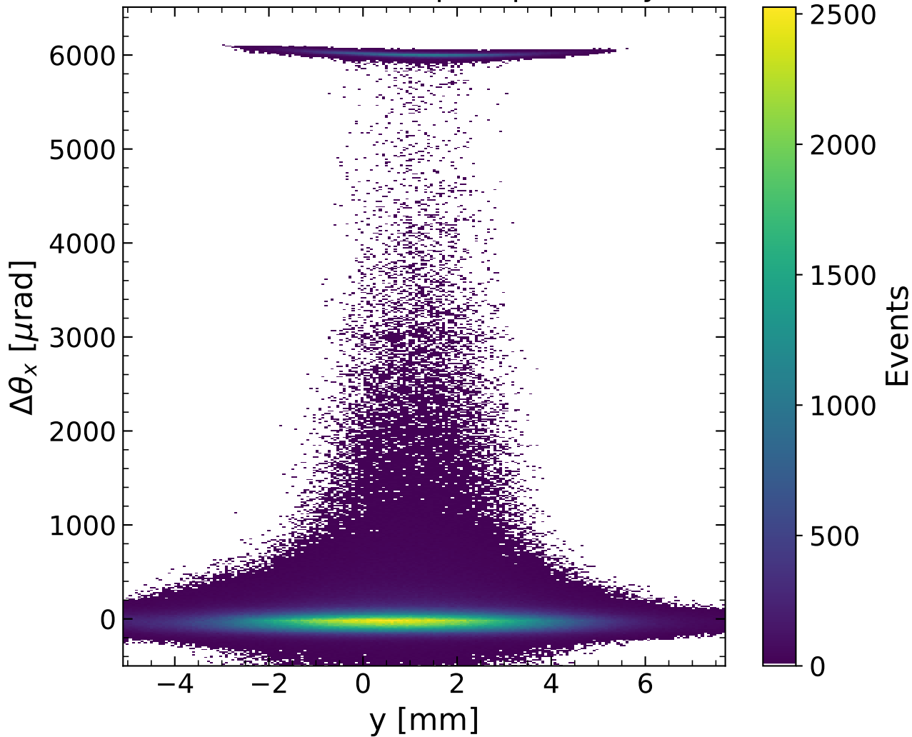
Deflection vs impact position y
