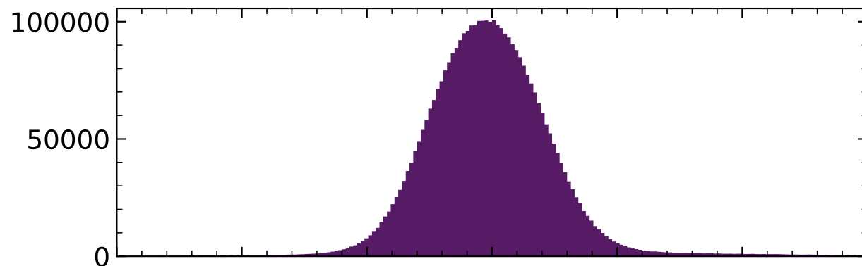
Incoming Angles Distribution
