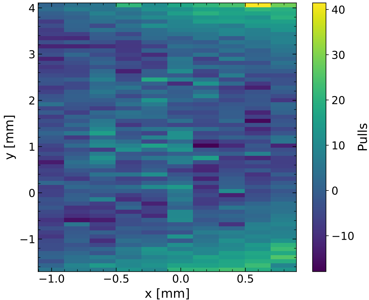
Torsion Pulls (data - fit) / \sigma
