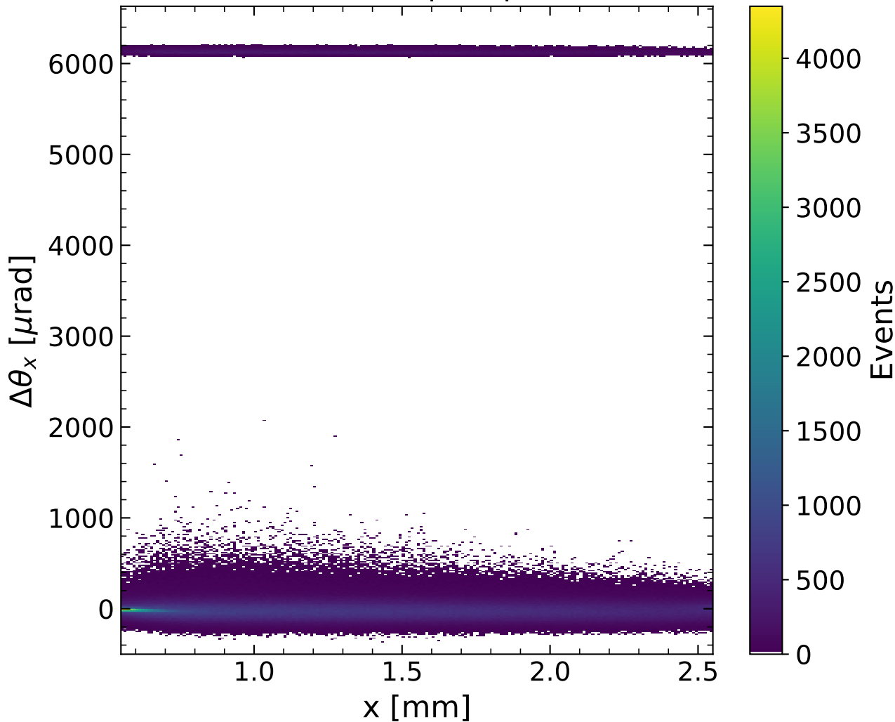
Deflection vs impact position x
