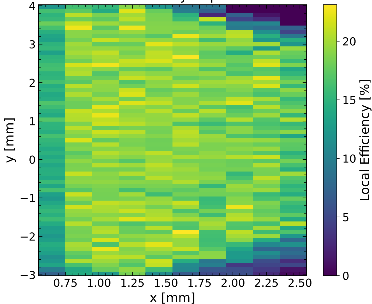
Efficiency Map
