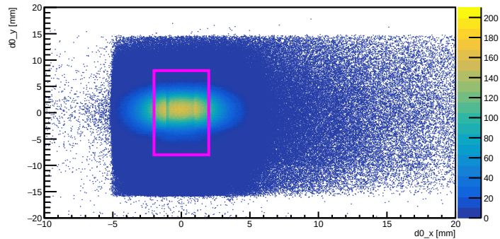
Outgoing d0\_x vs d0\_y of all particles
