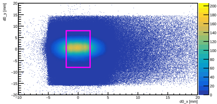
Incoming beam of all particles
