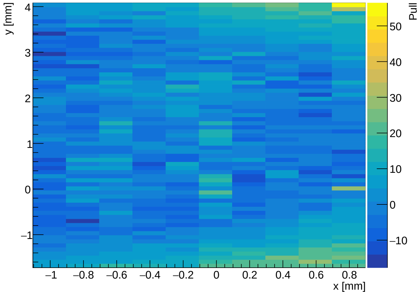
Torsion Pulls (Data - parabolic_y)/ \sigma
