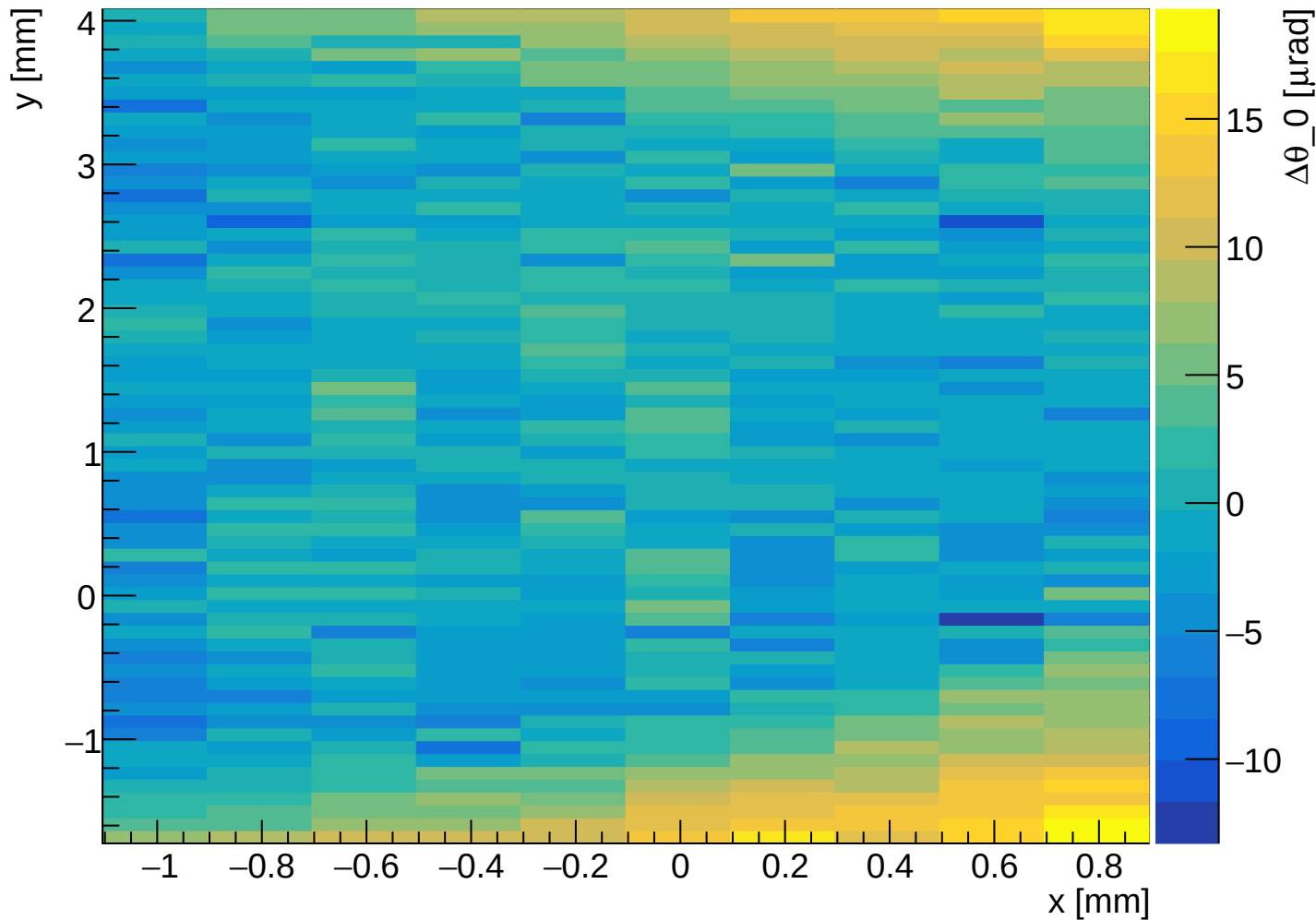
Torsion Residuals (Data - parabolic_y)
