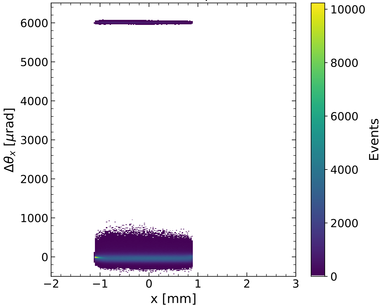
Deflection vs Impact X
