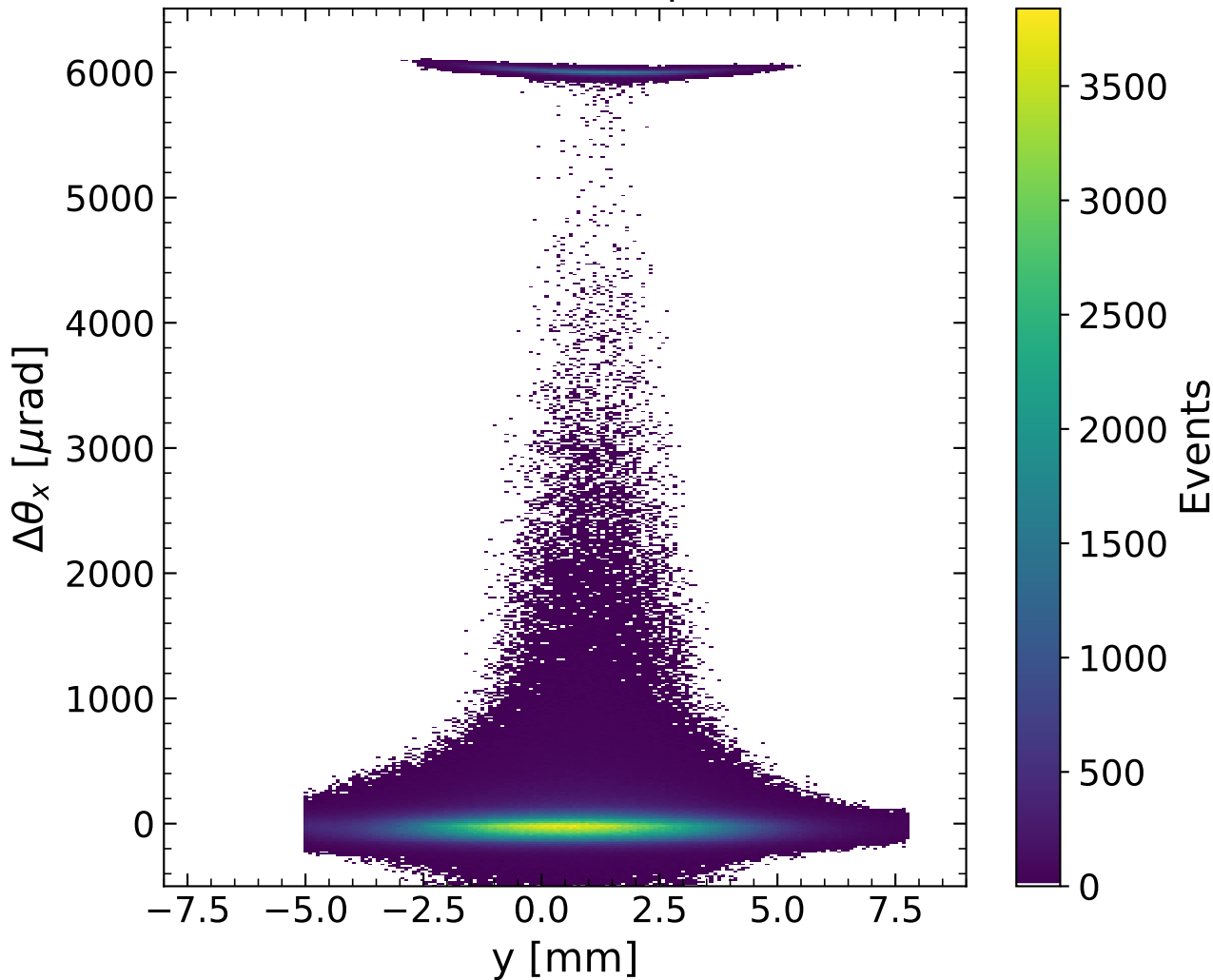
Deflection vs Impact Y
