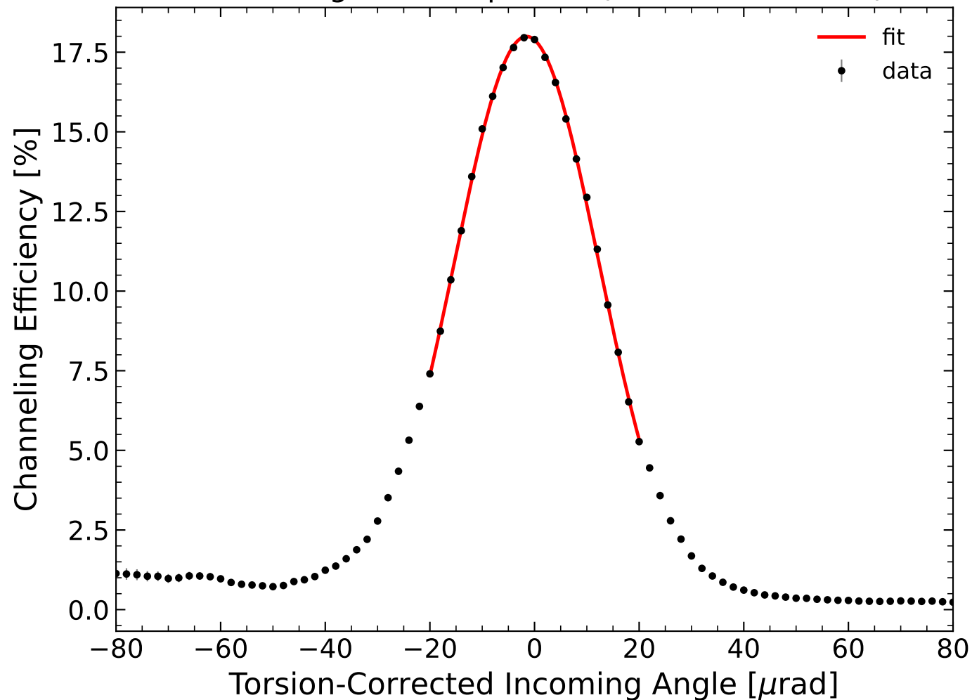
Global Angular Acceptance (Torsion Corrected)
