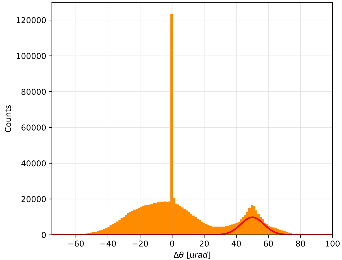
\Delta\theta distribution - (survived particles)
