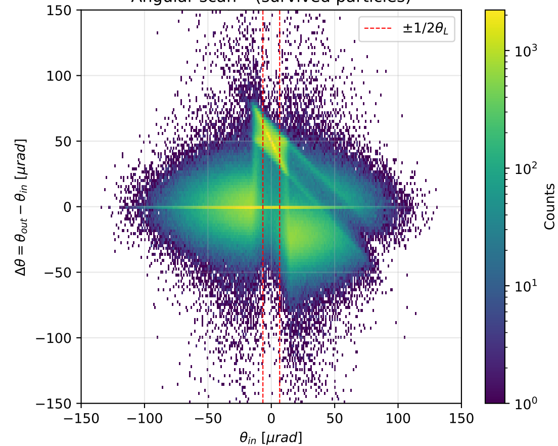
Angular scan - (survived particles)
