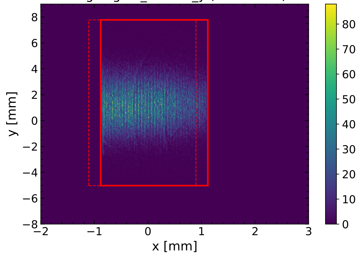
Outgoing d0_x vs d0_y (Channeled)
