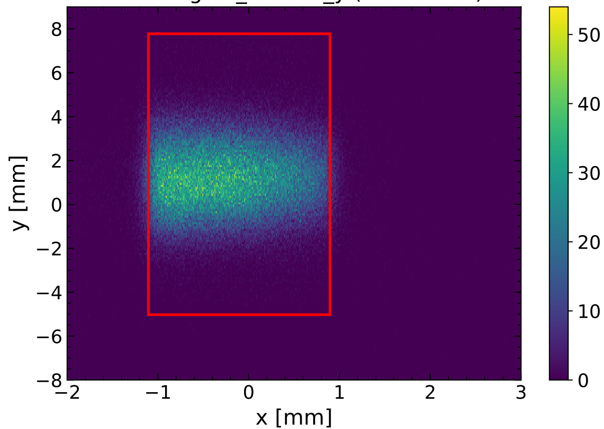
Incoming d0_x vs d0_y (Channeled)
