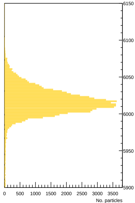
Angular Deflection cut at \pm \theta_L/2
