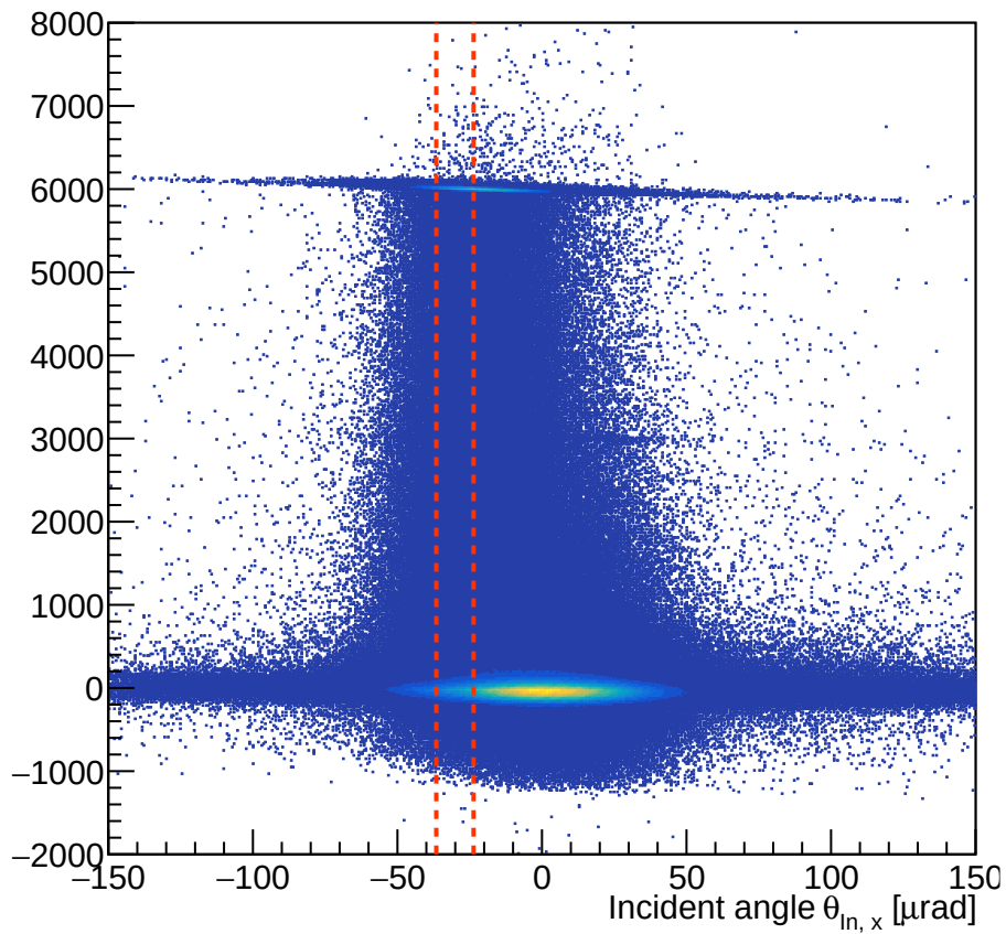
Angular deflection of the particles as a function of the incident angle
