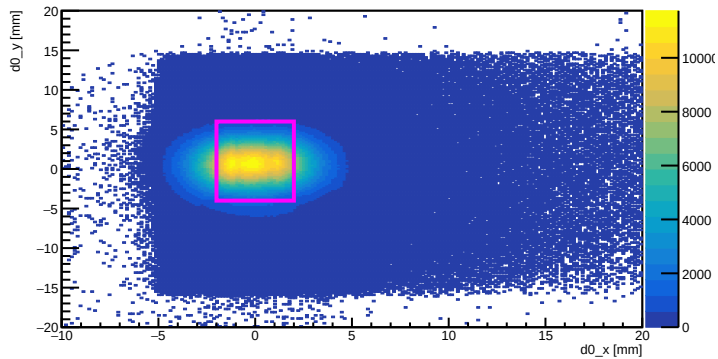
Incoming beam of all particles
