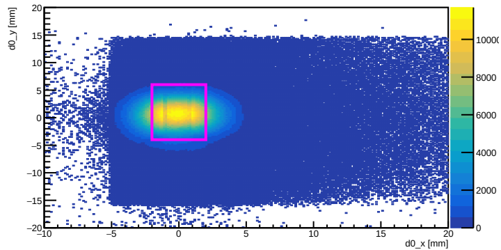
Outgoing d0\_x vs d0\_y of all particles
