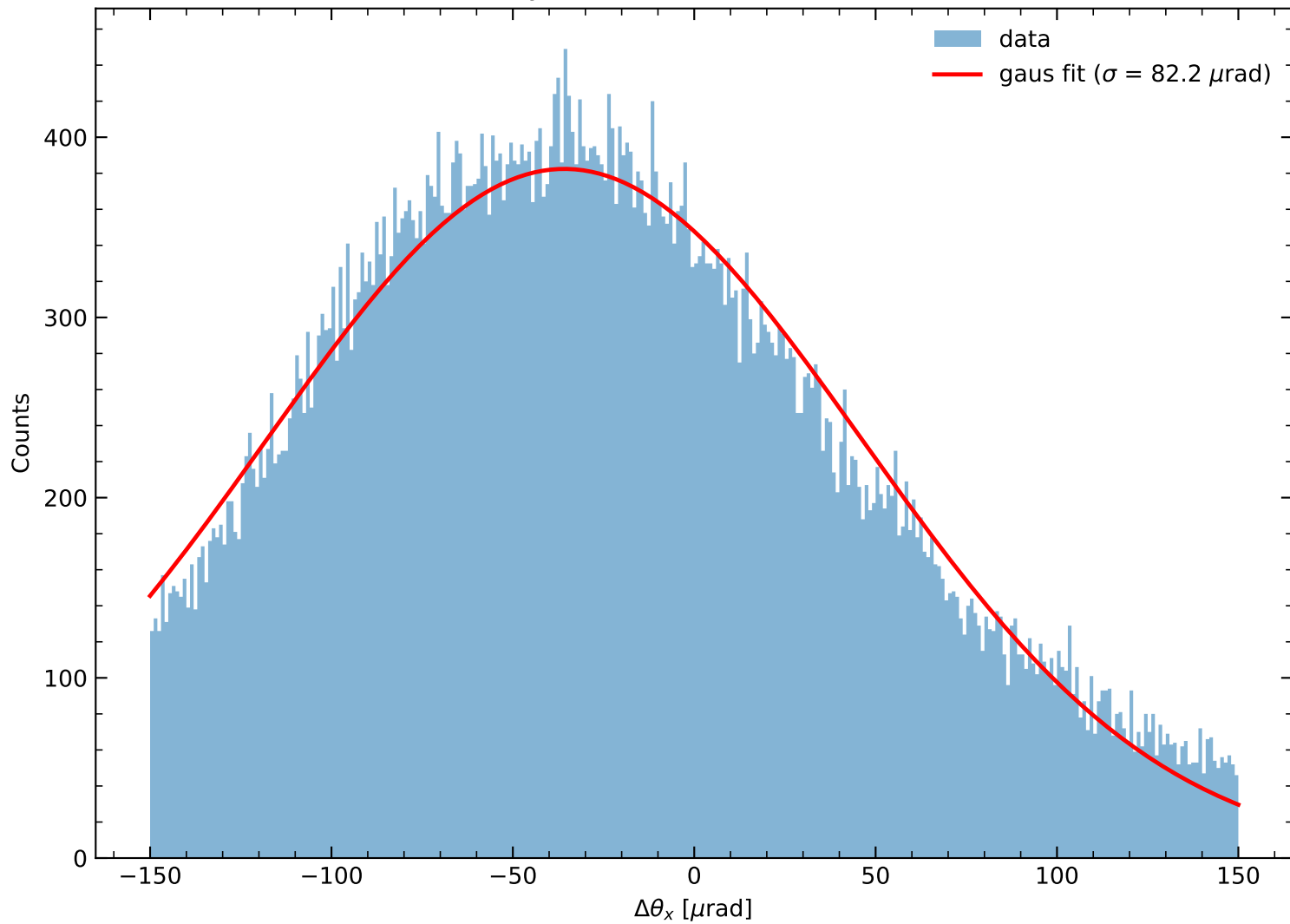
Crystal slice (X = -0.02 mm)
