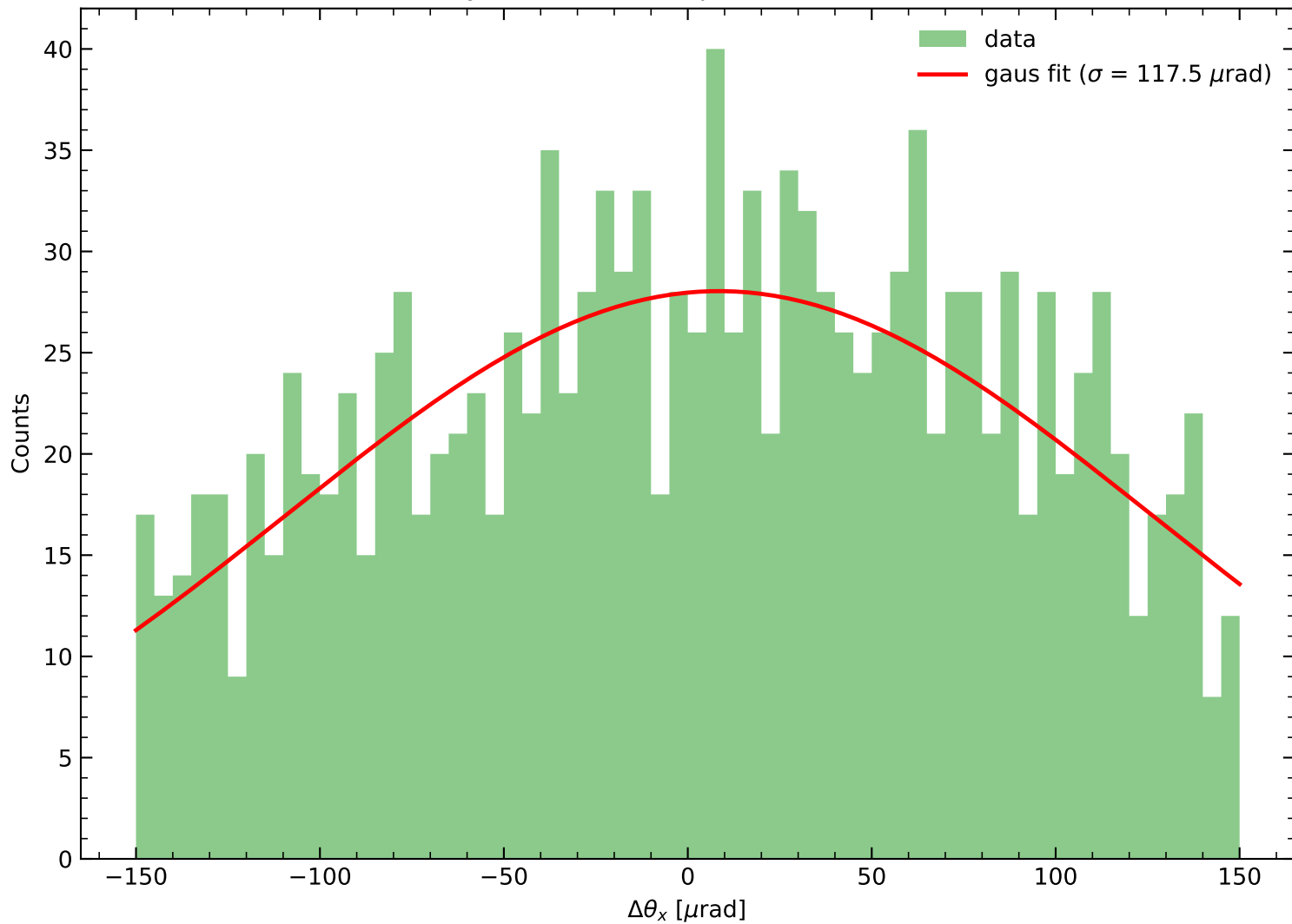
Crystal slice - clamp (Y = -9.90 mm)
