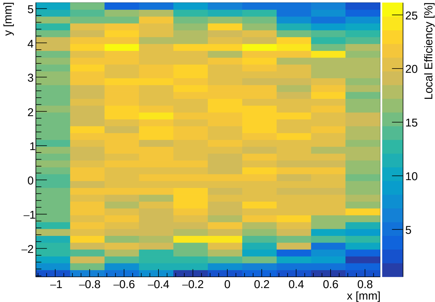
2D Efficiency Map
