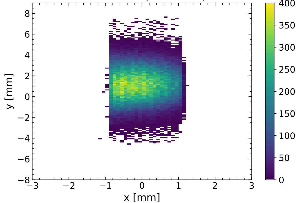
Downstream (Channeled)
