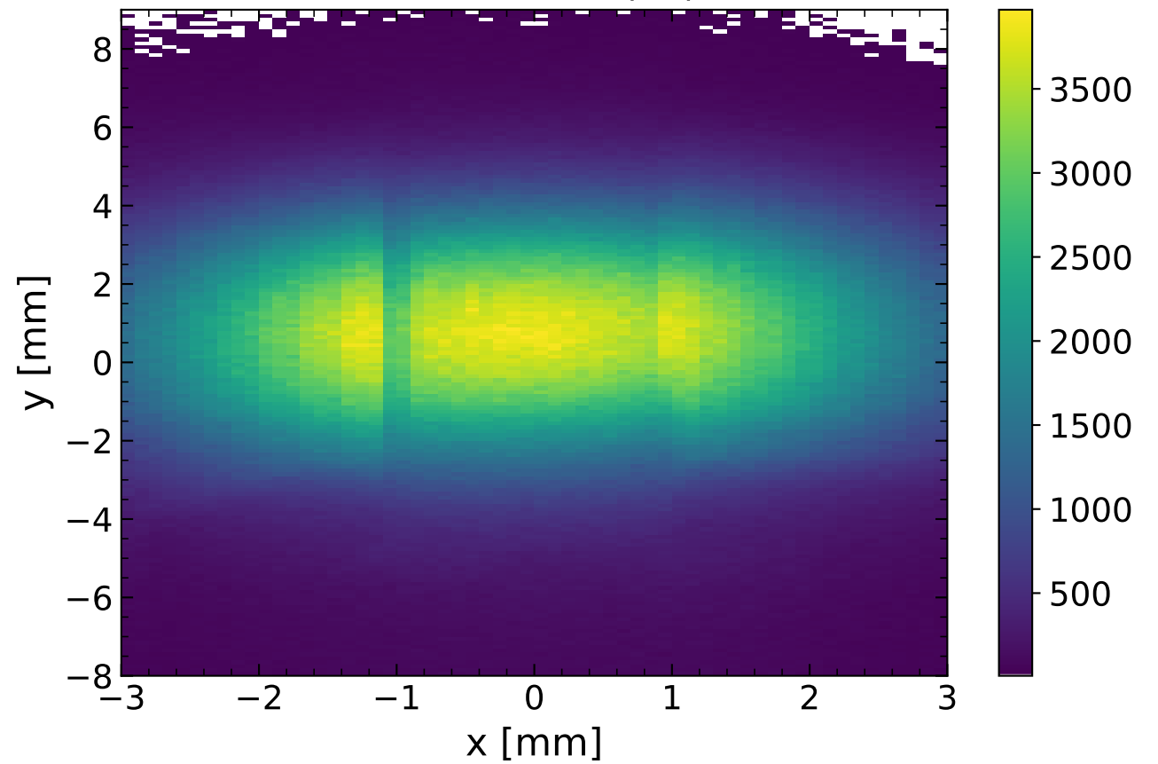
Downstream (Channeled)
