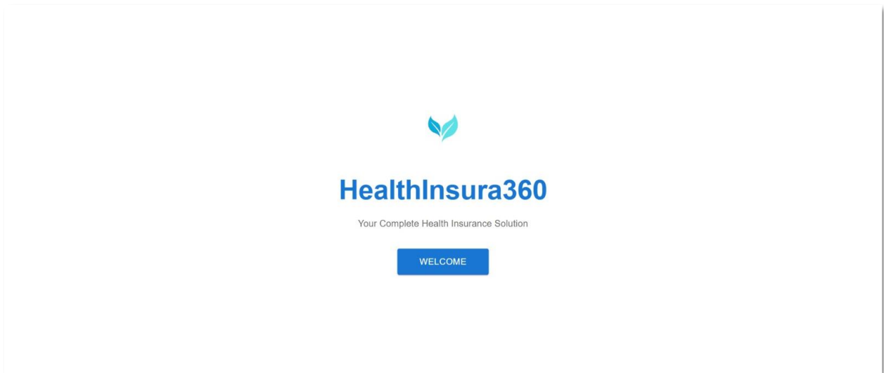
Figure 2. 3: Landing Page
