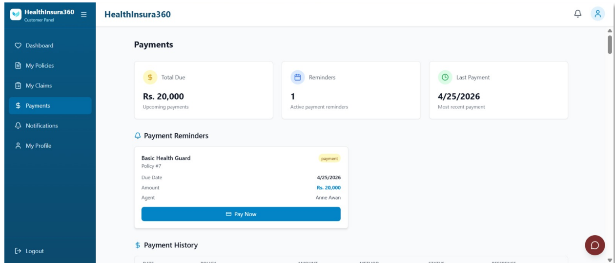
Figure 6. 7: User-Make Payments
