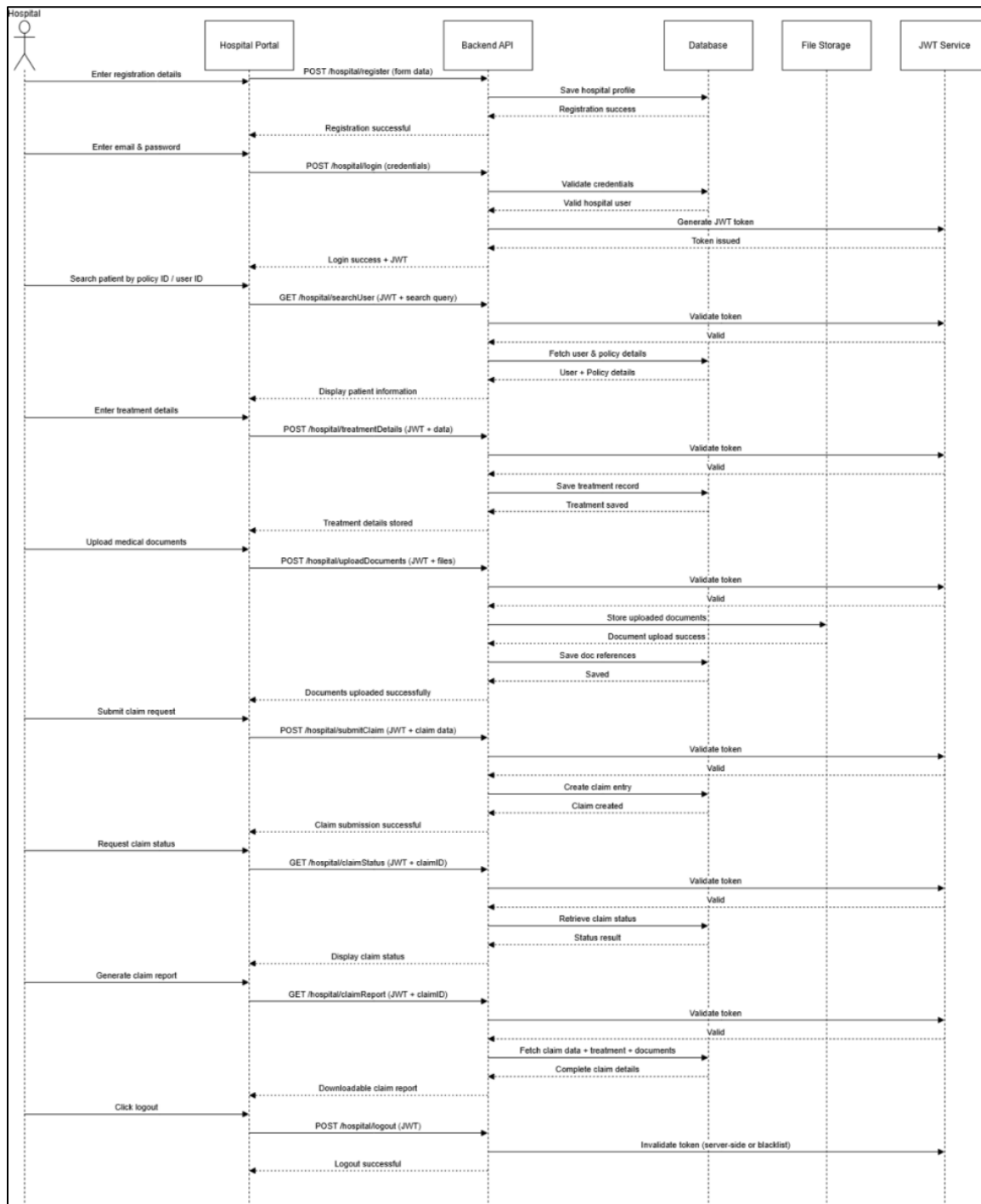
Figure 3. 11: Sequence Diagram of Hospital
