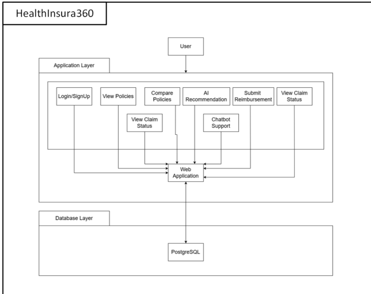
Figure 3. 1: User Package Diagram
