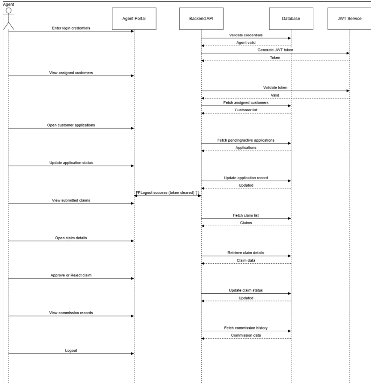
Figure 3. 10: Sequence Diagram of Agent
