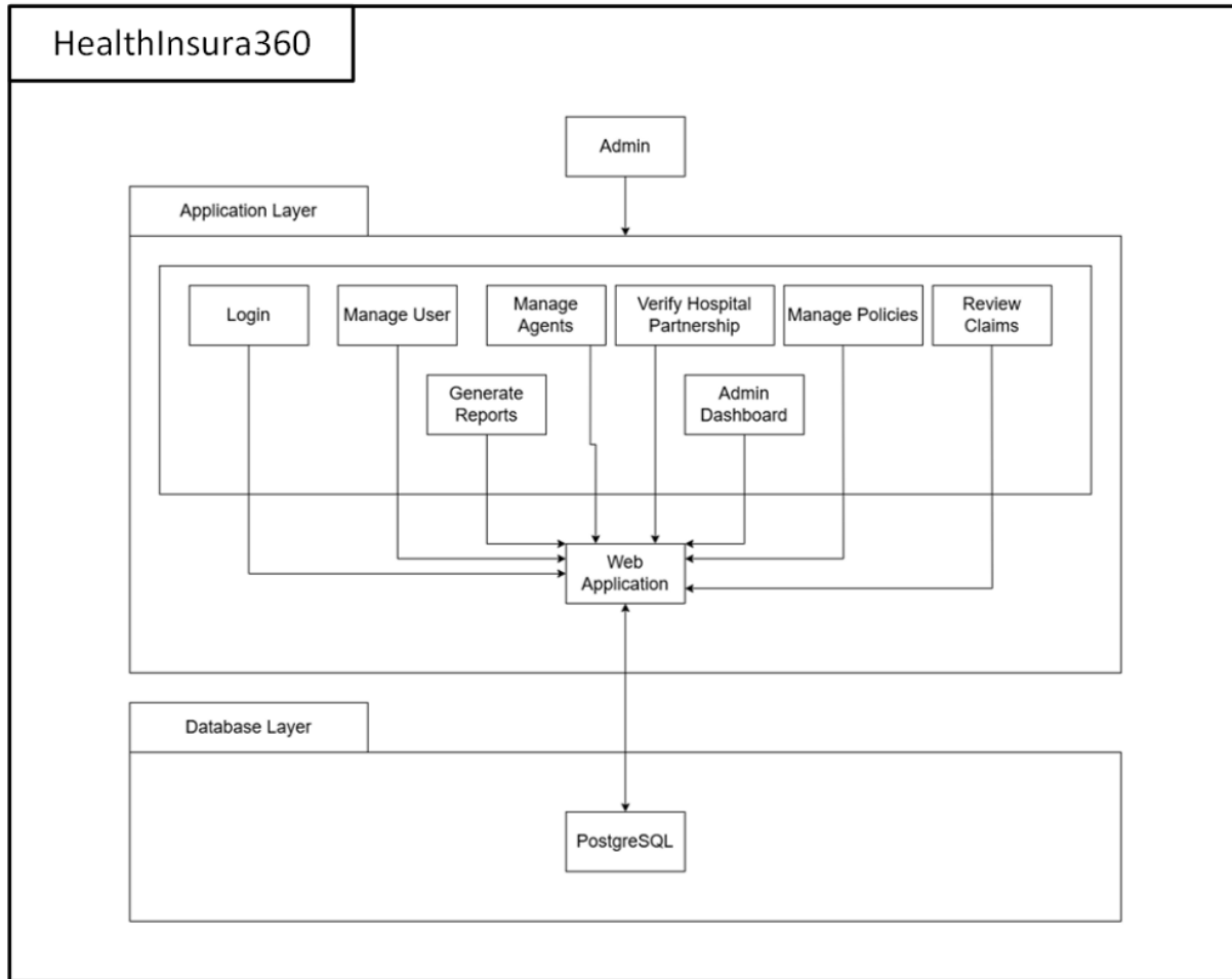
Figure 3. 2: Admin Package Diagram
