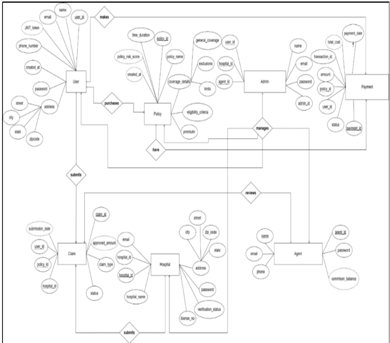
Figure 3. 7: Entity Relationship Diagram
