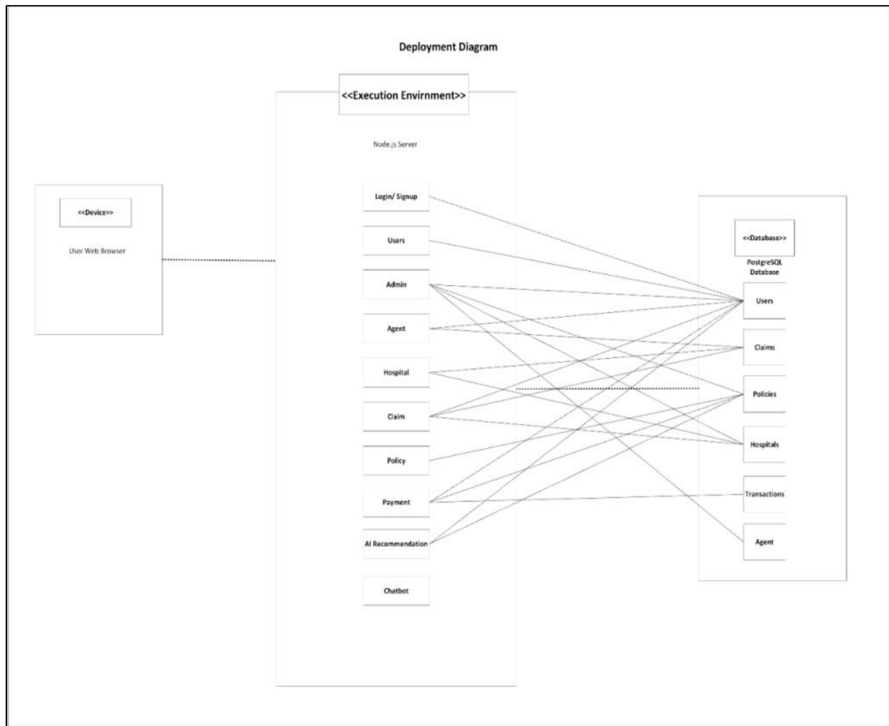
Figure 3. 5: Deployment Diagram
