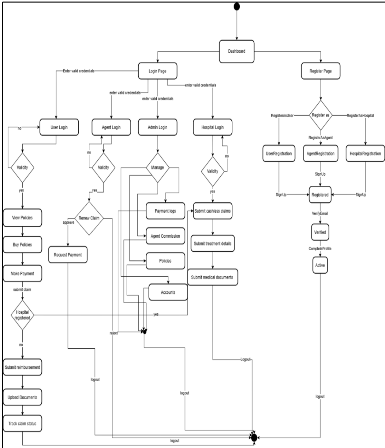
Figure 3. 12: State Machine Diagram
