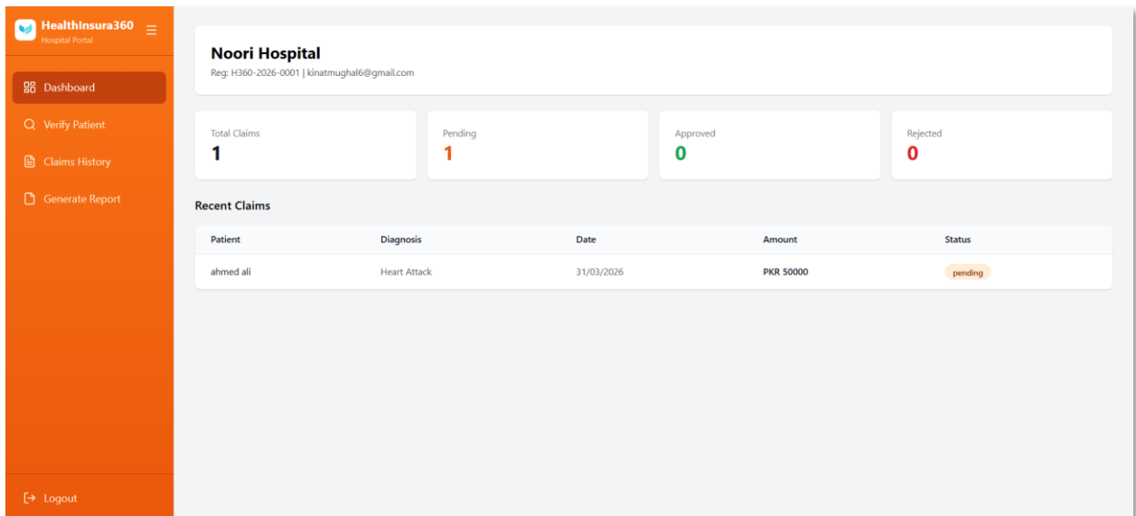
Figure 2. 8: Hospital Screen
