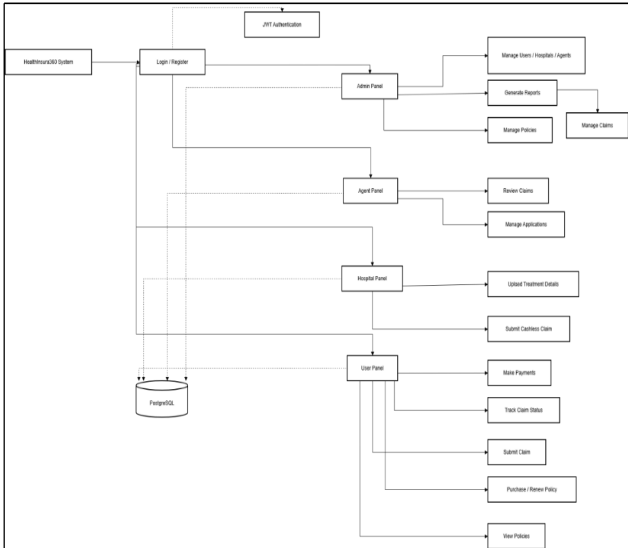
Figure 2. 1: System Design
