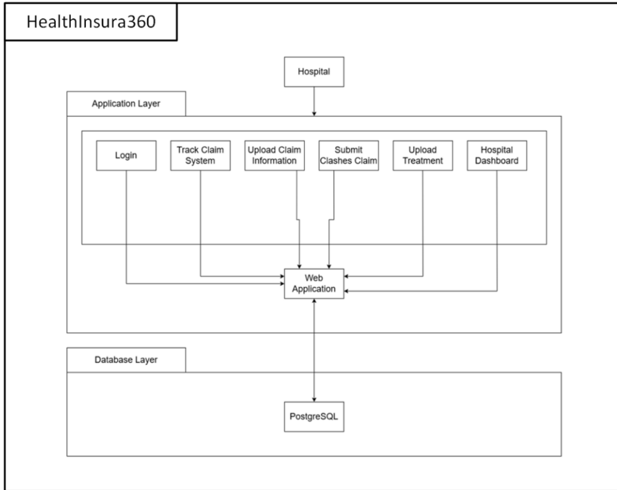
Figure 3. 3: Hospital Package Diagram
