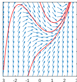
Direction field + integral curves
