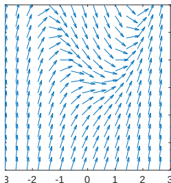
All vectors equal length
