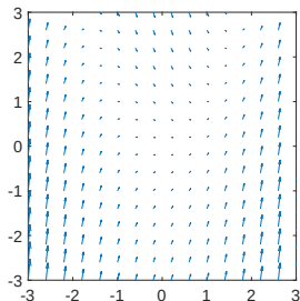
All vectors equal \Delta x
