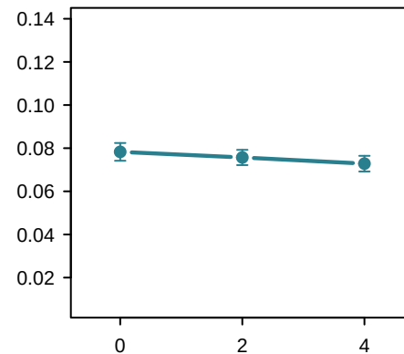
autocorrelation (patch SD 2)
