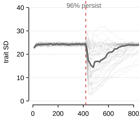
96% persist
