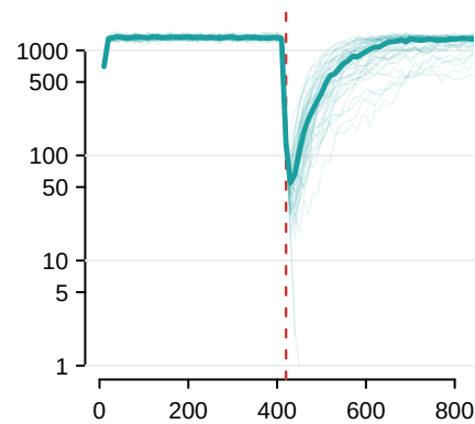
rough, correlated
