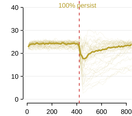
100% persist
