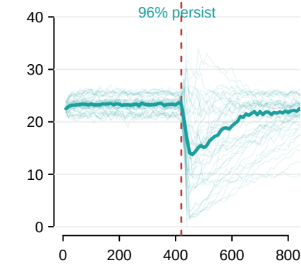
96% persist
