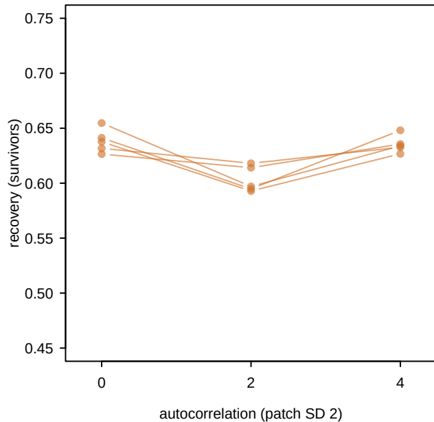
five landscape replicates agree
