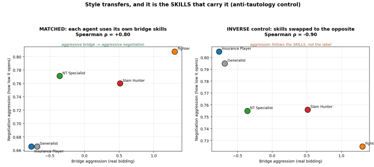
Fig. 5. Inverse-prompt control. Swapping each profile’s bridge-derived skills (labels unchanged) flips the alignment from +0.80 to -0.90 : the behavior follows the skills, not the label.
