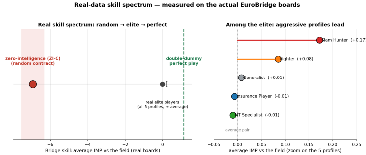
Fig. 2. The validated skill spectrum: the ZI-C random baseline loses \sim 7 IMP/board to the field; elite profiles cluster near the datum; the double-dummy oracle gains +1.1 . A metric that cannot reproduce this ordering is measuring the wrong thing.
