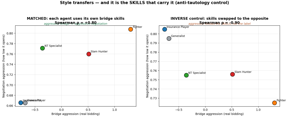
Figure 2.4: Matched skills (left, +0.80 ) vs. swapped skills (right, -0.90 ): the skills carry the style.
