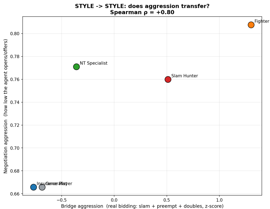
Figure 2.3: Style ↔ style: bridge aggression (real bidding) vs. negotiation aggression (how low the agent opens), \rho = +0.80 .
