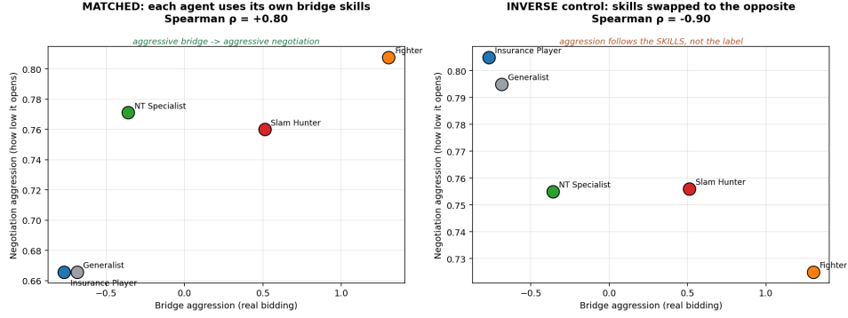
Figure 5: Inverse-prompt control. Swapping each profile’s bridge-derived skills (labels unchanged) flips the alignment from +0.80 to -0.90 : the behavior follows the skills, not the label.
