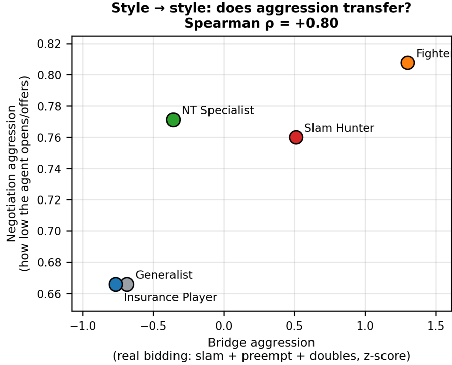
Fig. 4. Behavioral alignment: bridge-derived aggression ( x ) vs. negotiation demand depth ( y ), \rho_S = +0.80 .
