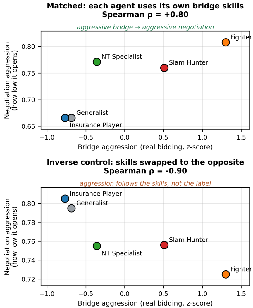
Fig. 5. Inverse-prompt control. Swapping each profile’s bridge-derived skills (labels unchanged) flips the alignment from +0.80 to -0.90 : the behavior follows the skills, not the label.
