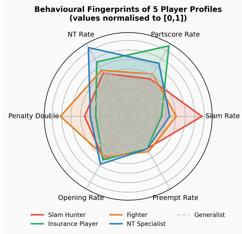
Fig. 1. Behavioral fingerprints of the four extreme profiles against the Generalist baseline (each feature min–max normalized to [0,1] across all players). Each profile is extreme on its own defining axis, and only mildly deviant elsewhere.
