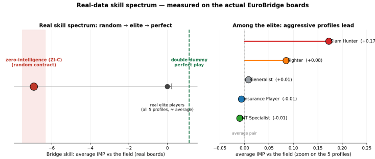
Fig. 2. The validated skill spectrum: the ZI-C random baseline loses \sim 7 IMP/board to the field; elite profiles cluster near the datum; the double-dummy oracle gains +1.1. A metric that cannot reproduce this ordering is measuring the wrong thing.
