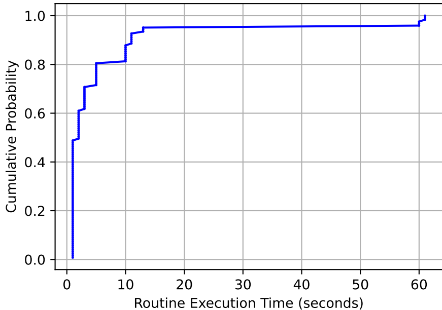
CDF of Routine Action Lengths
