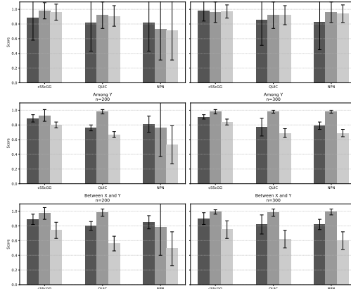
Figure 3: Comparison of SPE (dark), SEN (gray), and F1 (light) scores among and between \mathbf{X} and \mathbf{Y} for different methods for the non-Gaussian case (27) with c_1 = 1 and c_2 = 1 .
