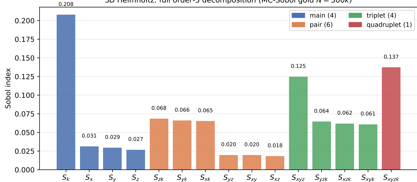
3D Helmholtz: full order-3 decomposition (MC-Sobol gold N = 300k )
