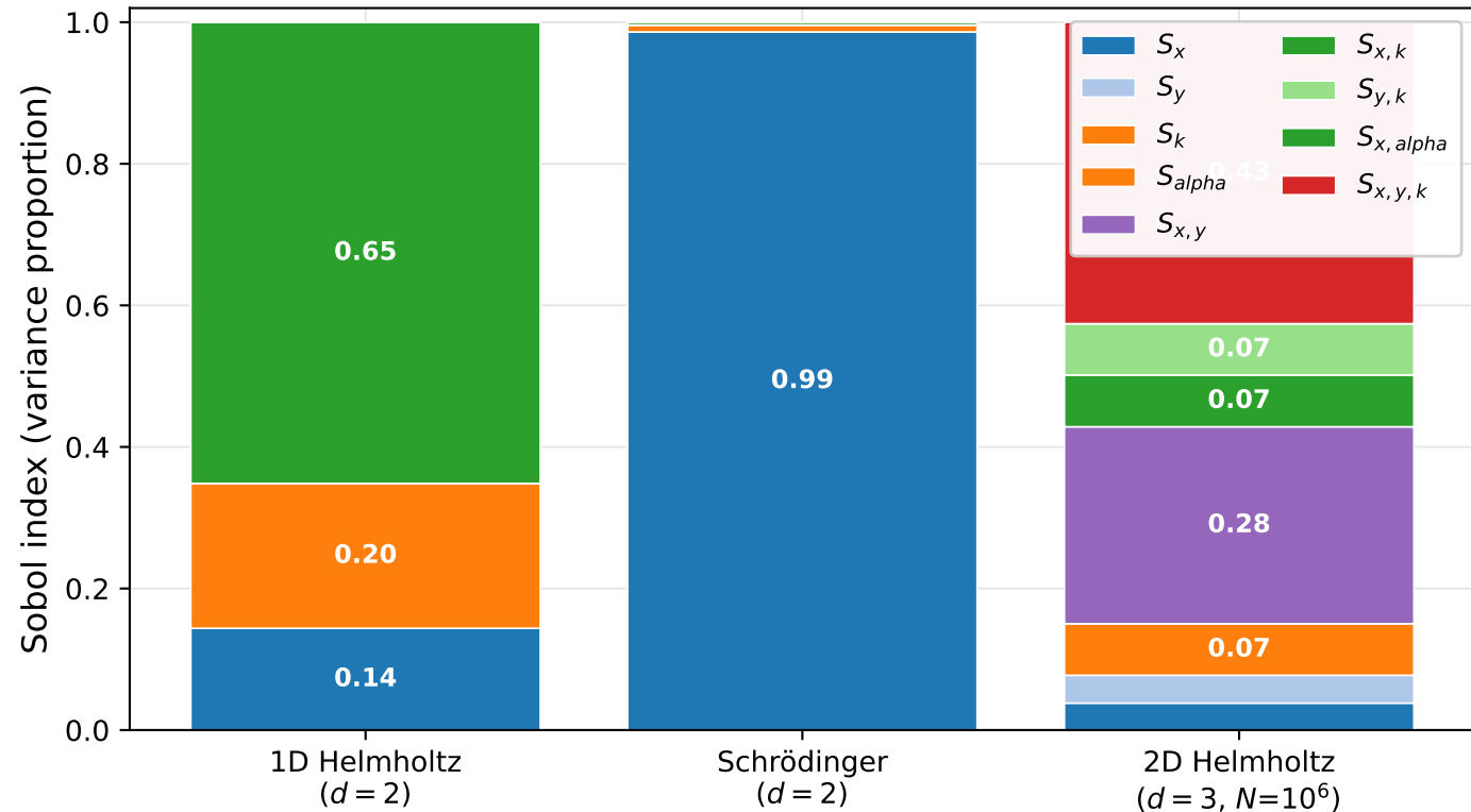
Functional-ANOVA Sobol decomposition across three parametric PDEs
